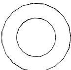
H100497 RONDELLE PLATE (x1) 17 x 30 BLK
